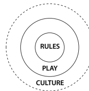
Primary Schemas
